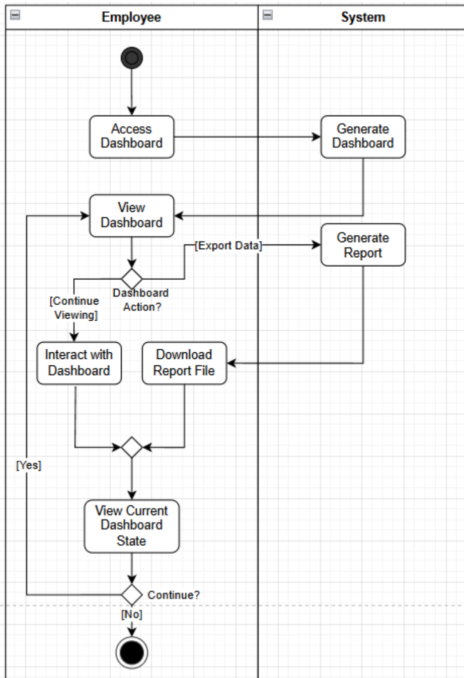
Activity Diagram for UC-14 (View Dashboard – Employee)
