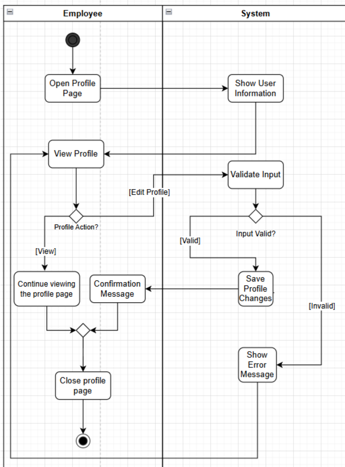
Activity Diagram for UC-03 (Edit User Profile - Employee)
