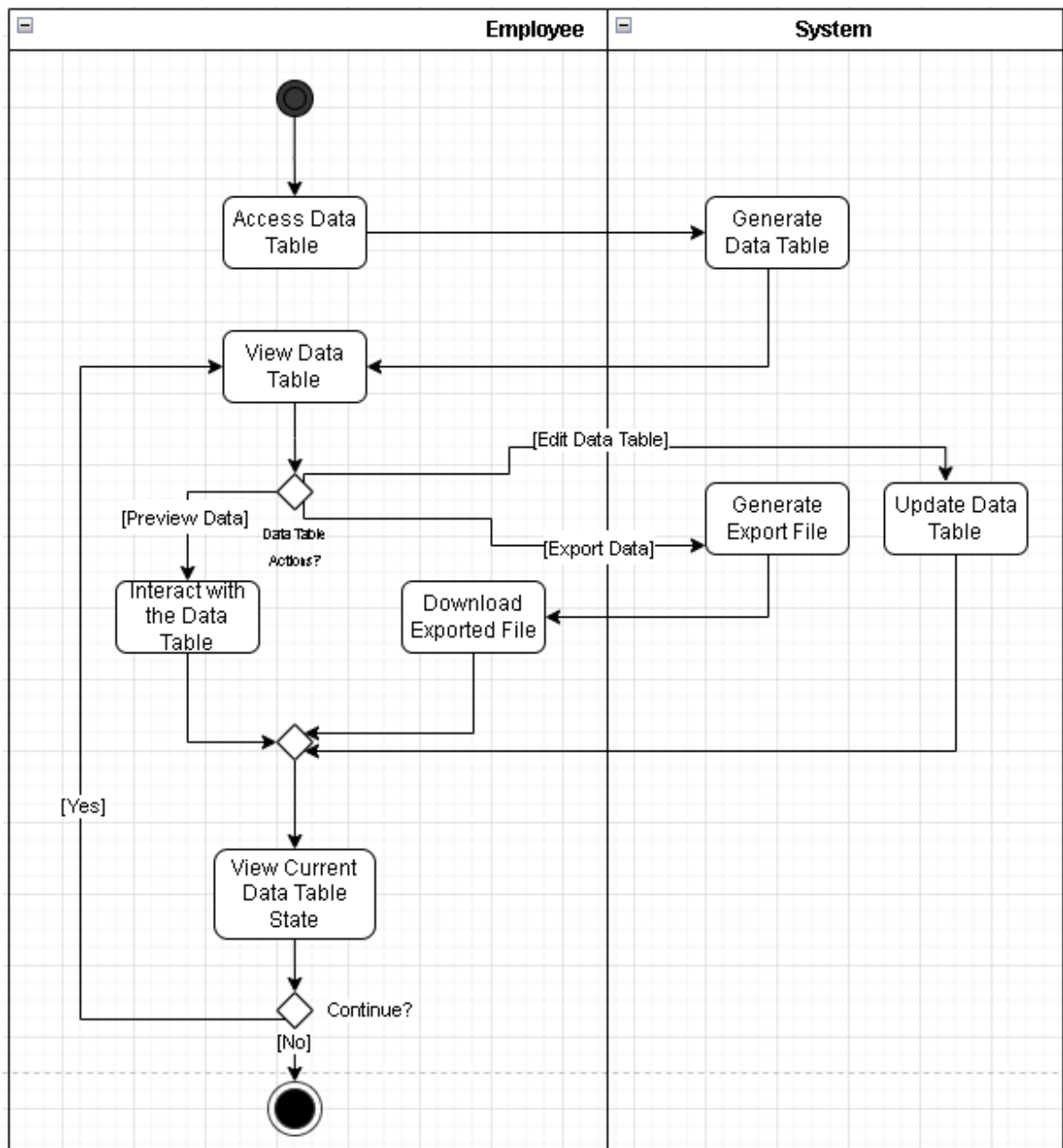
Activity Diagram for UC-05 (Manage Data Table)
