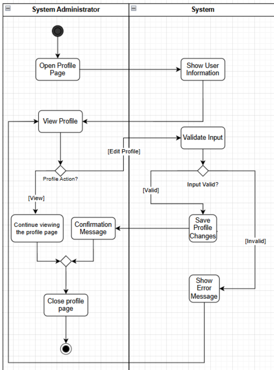
Activity Diagram for UC-15 (Edit User Profile – System Administrator)
