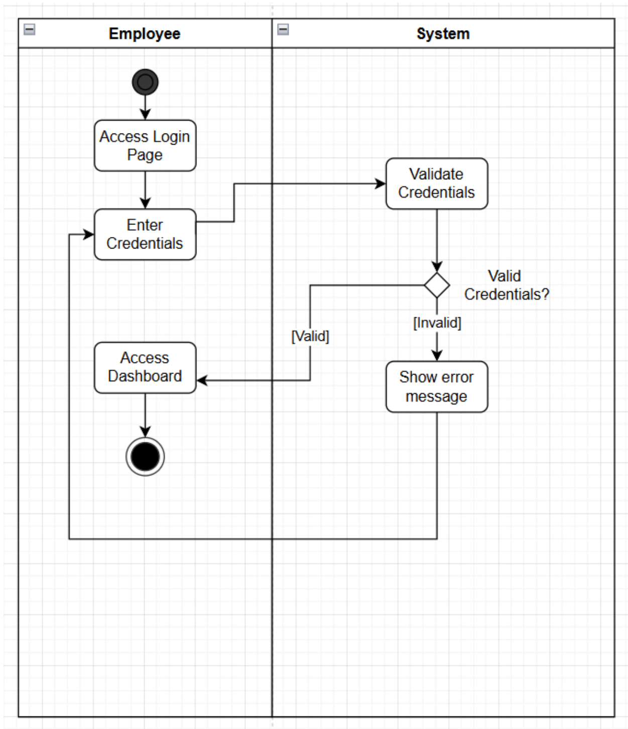
Activity Diagram for UC-02 (Login)
