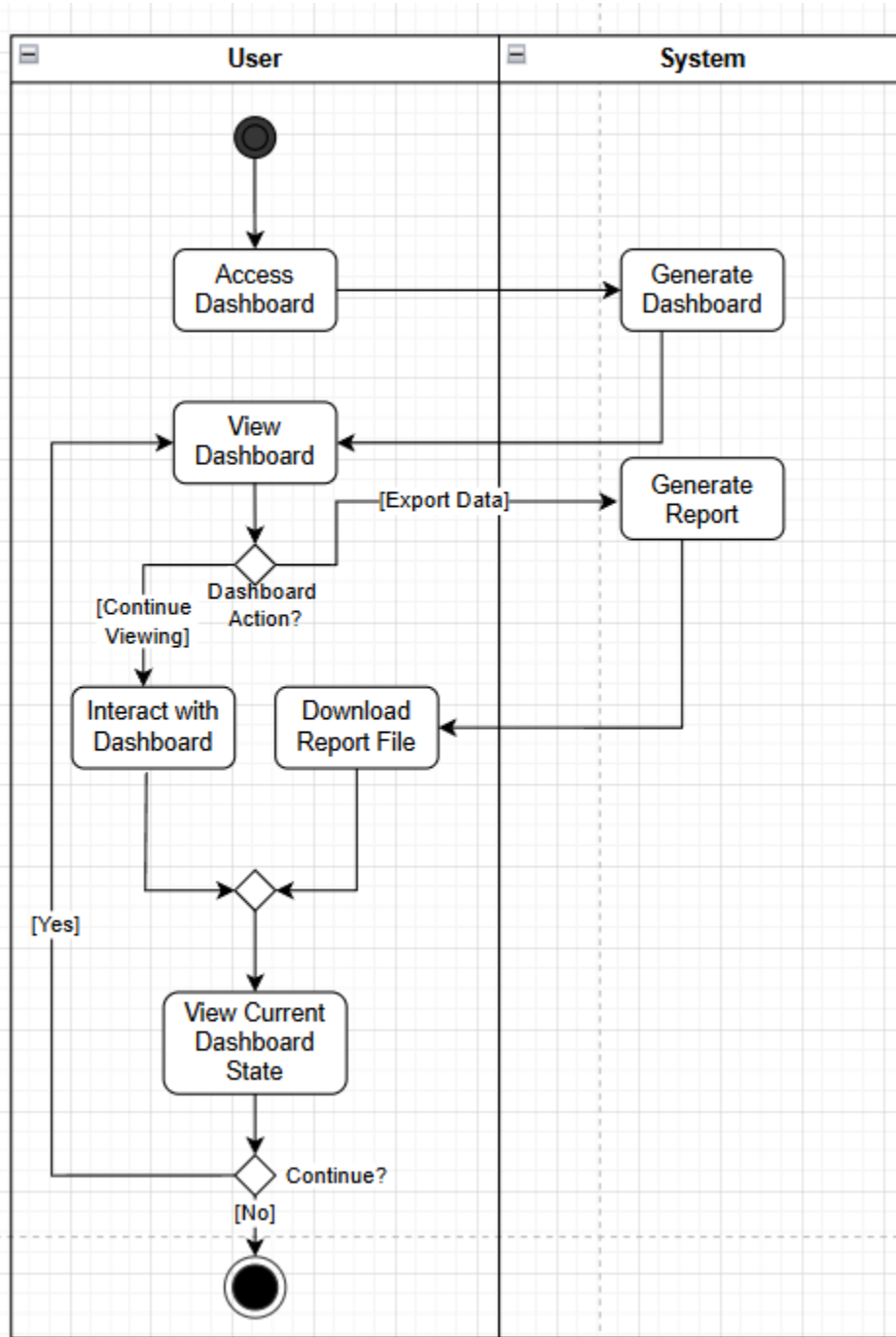
Activity Diagram for UC-04 (View Dashboard - User)
