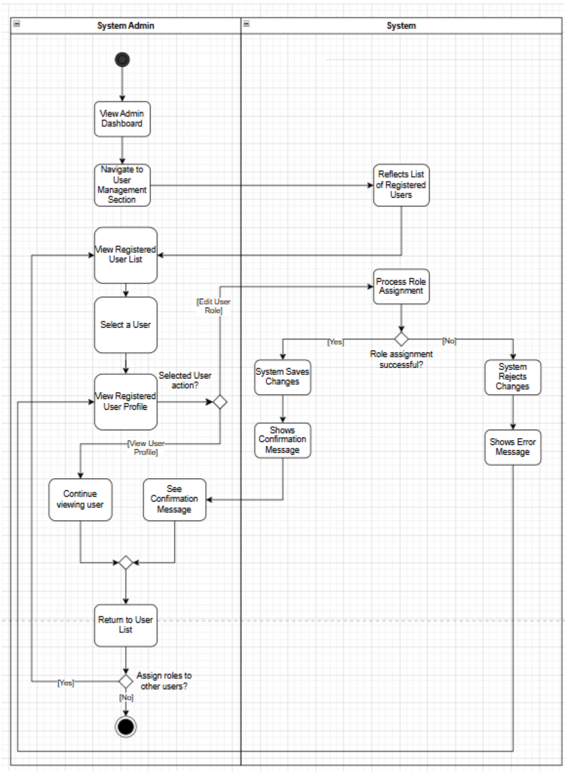
Activity Diagram for UC-08 (Assign Roles)
