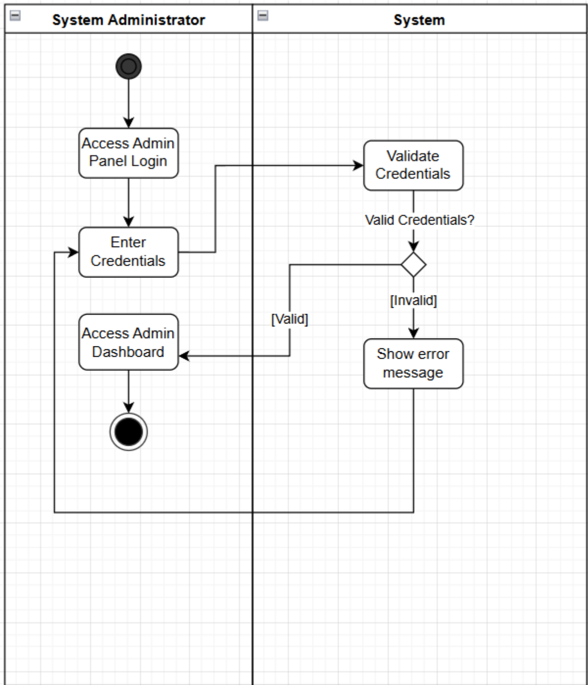
Activity Diagram for UC-07 (Administrator Panel Login)
